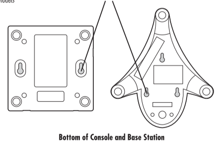
Bottom of Console and Base Station
