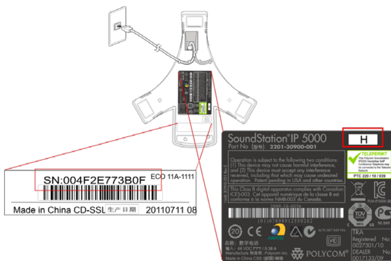
Figure 2: Label on Bottom of SoundStation IP 5000 Conference Phone
