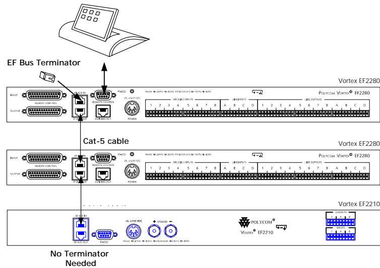
Figure 5. Only the EF2280 needs to be terminated when linked together with EF2211/EF2210s.
