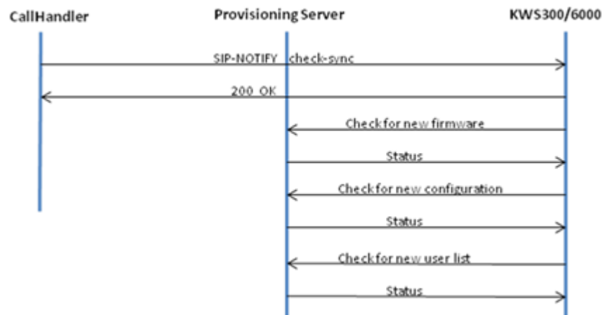
Figure -3 Receiving SIP NOTIFY check-sync
